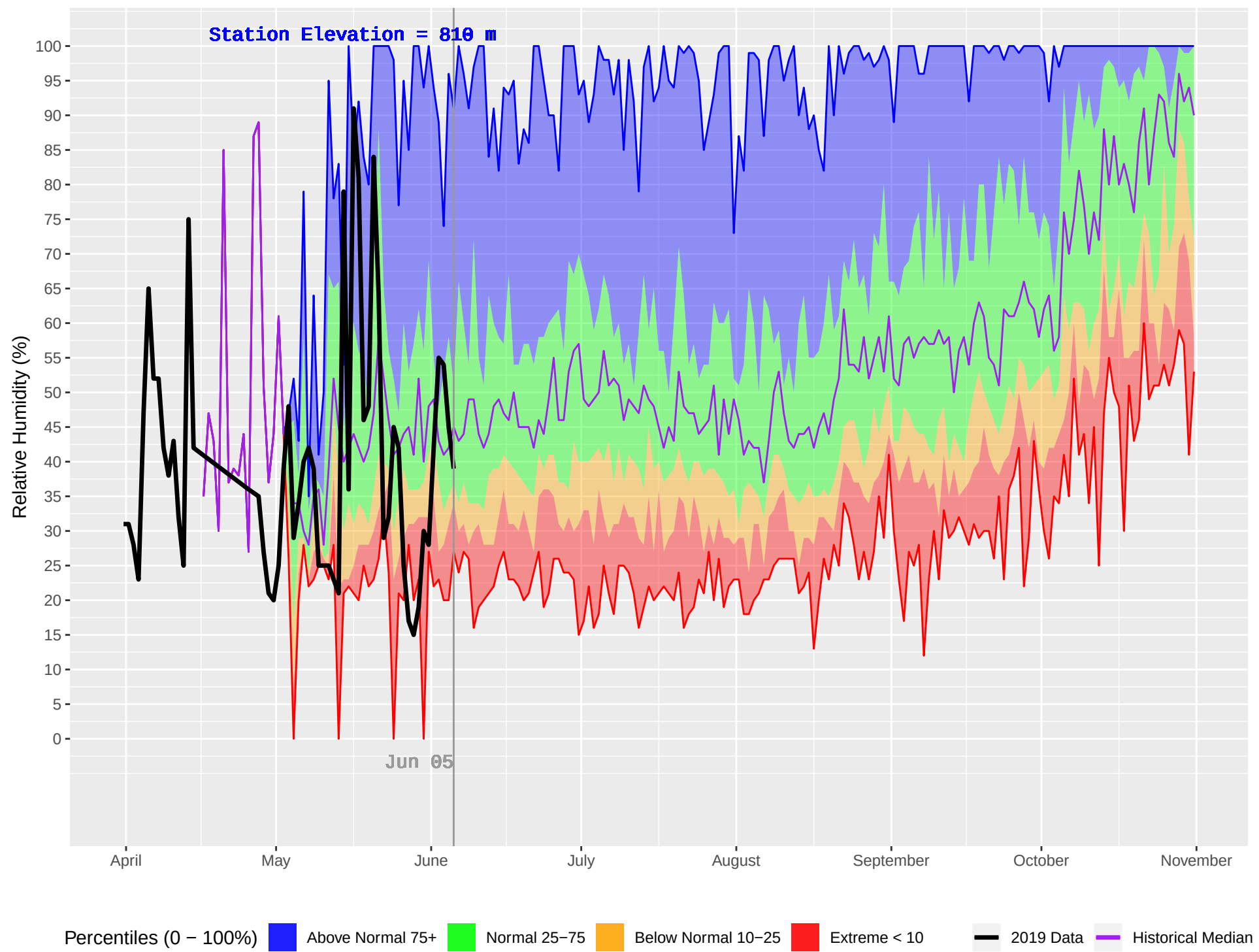
MCBRIDE LAKE (180) : Historical (1990–2018) and Current (2019) Daily Relative Humidity
