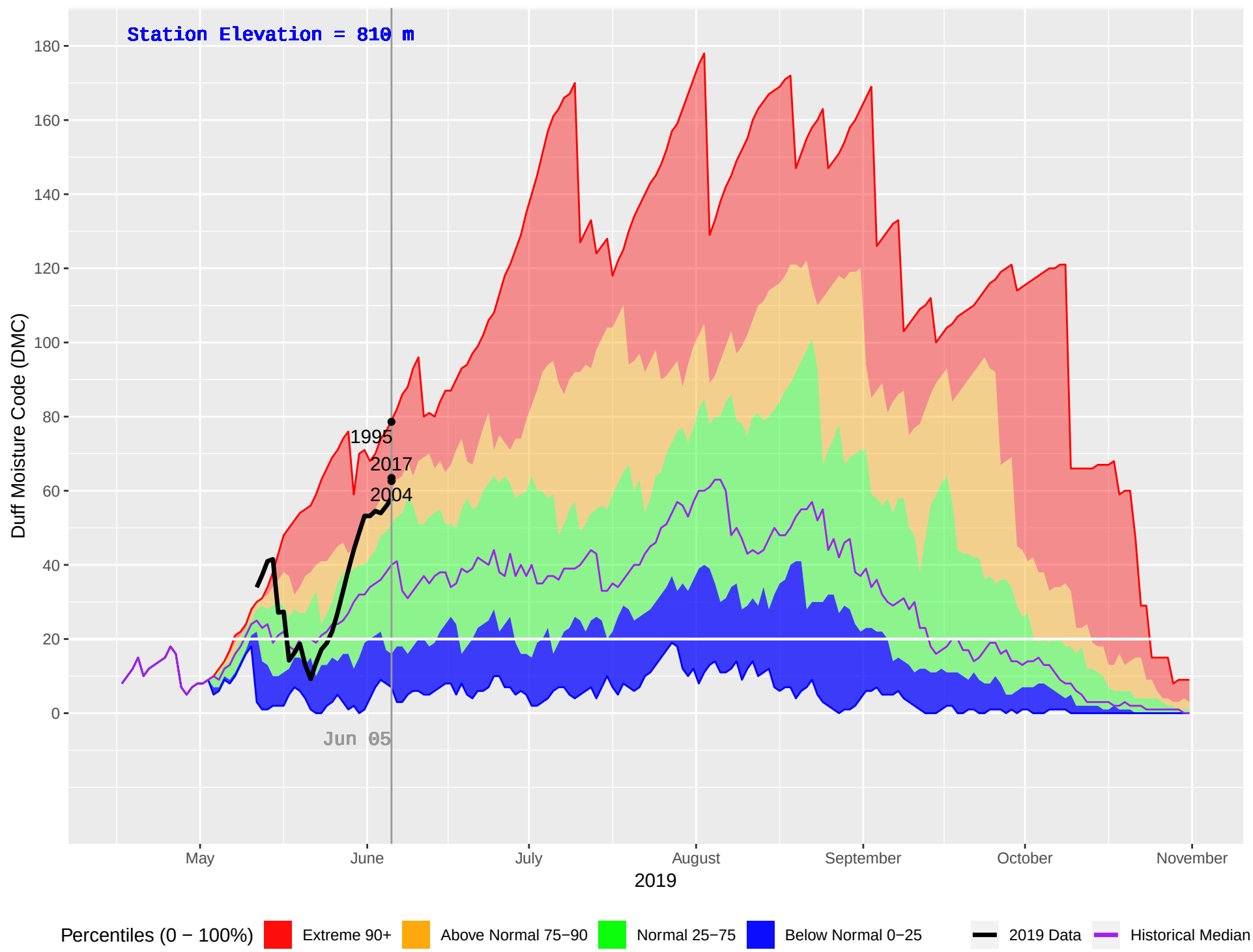
MCBRIDE LAKE (180) : Historical (1990–2018), Current (2019) Daily Duff Moisture Code (DMC)
