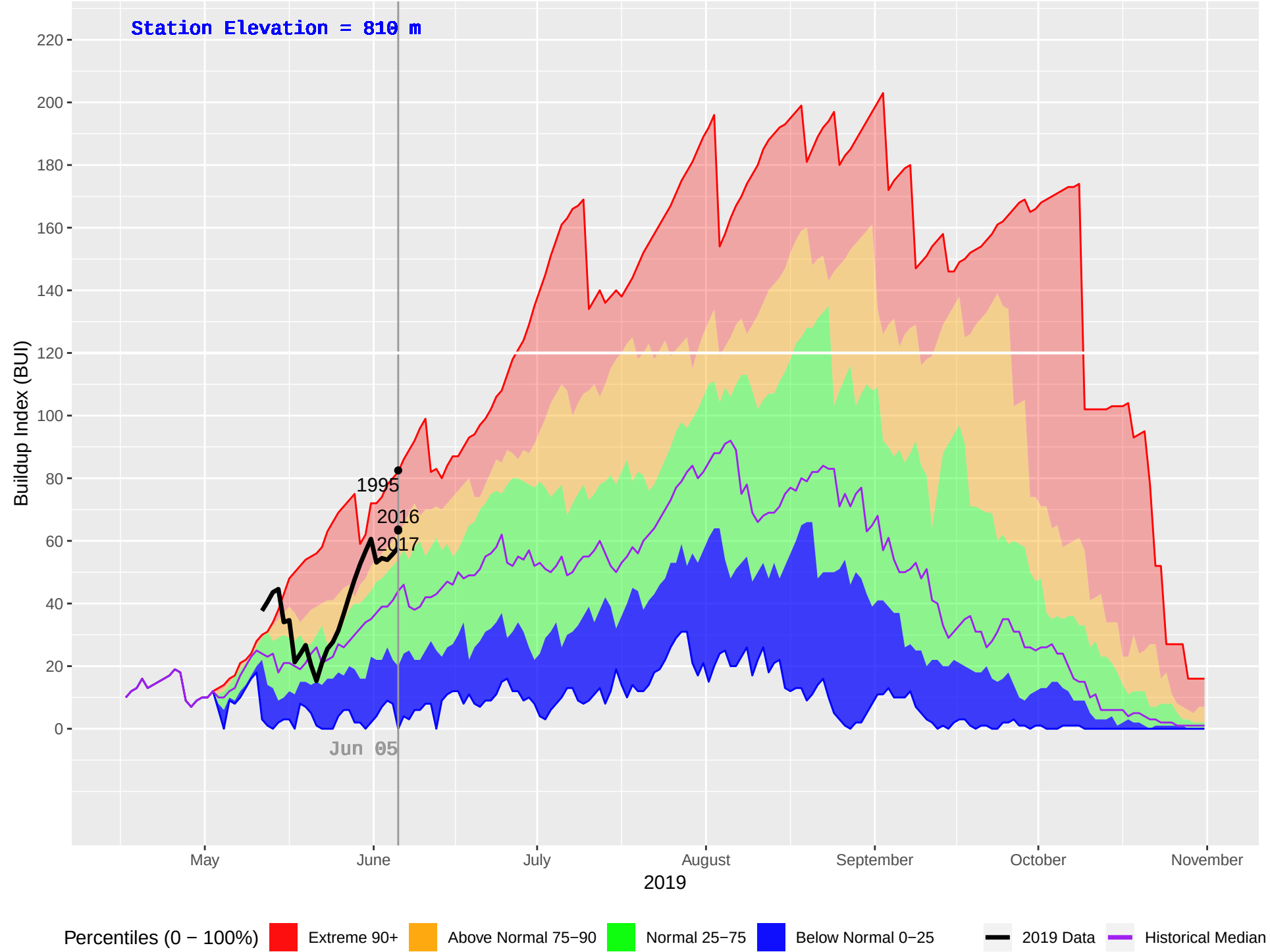
MCBRIDE LAKE (180) : Historical (1990–2018), Current (2019) Daily Buildup Index (BUI)
