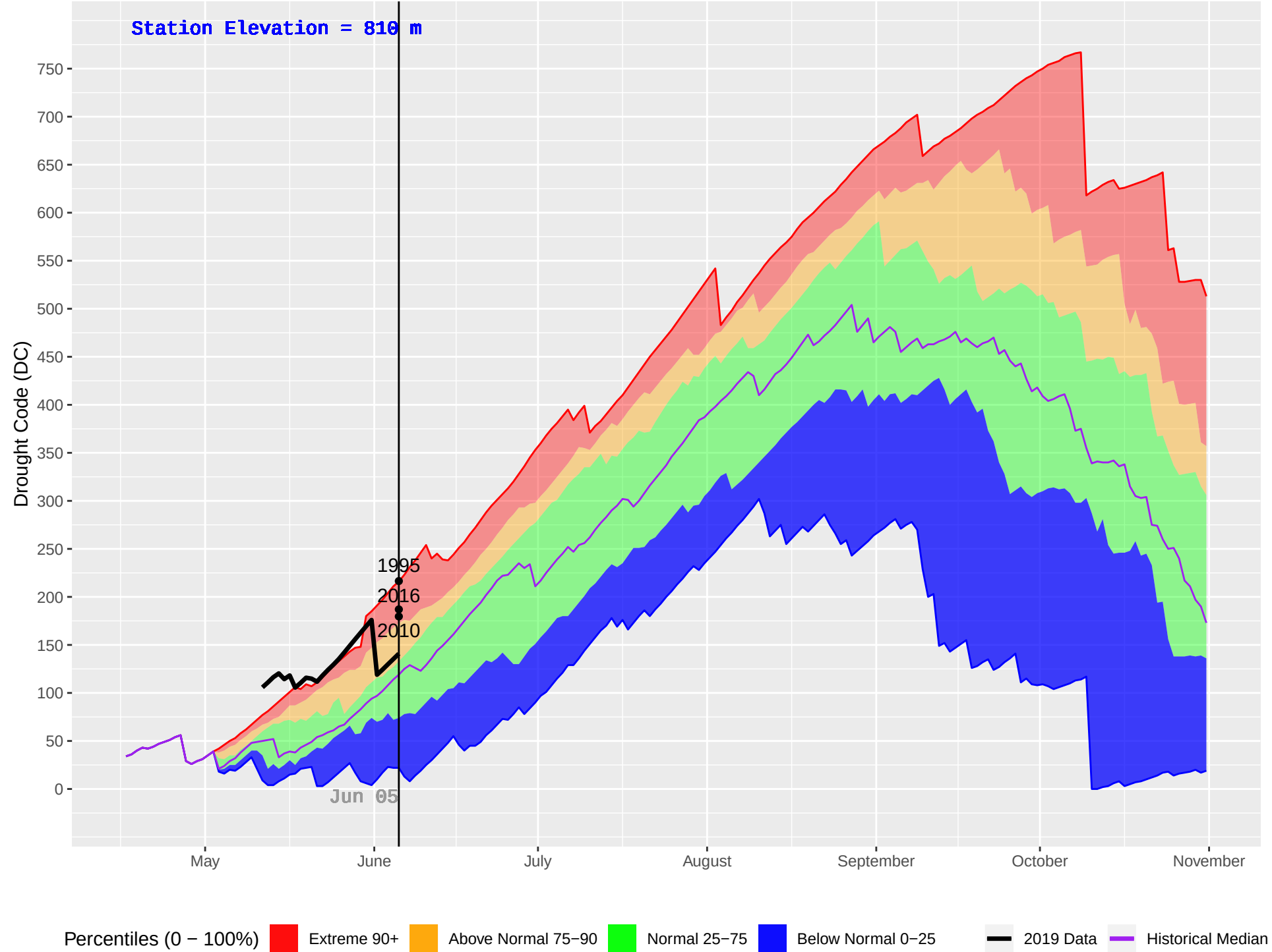
MCBRIDE LAKE (180) : Historical (1990–2018) and Current (2019) Daily Drought Code (DC)
