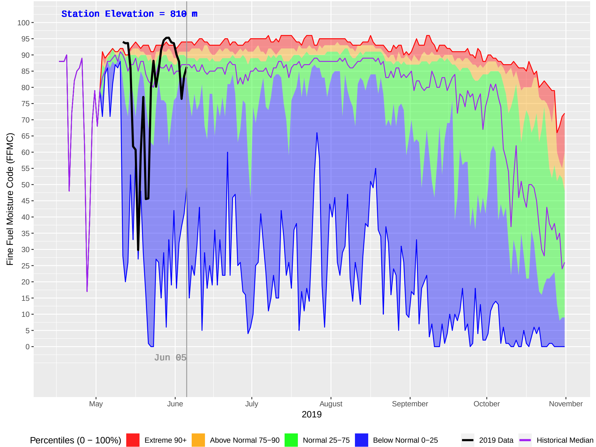
MCBRIDE LAKE (180) : Historical (1990–2018) and Current (2019) Daily Fine Fuel Moisture Code (FFMC)
