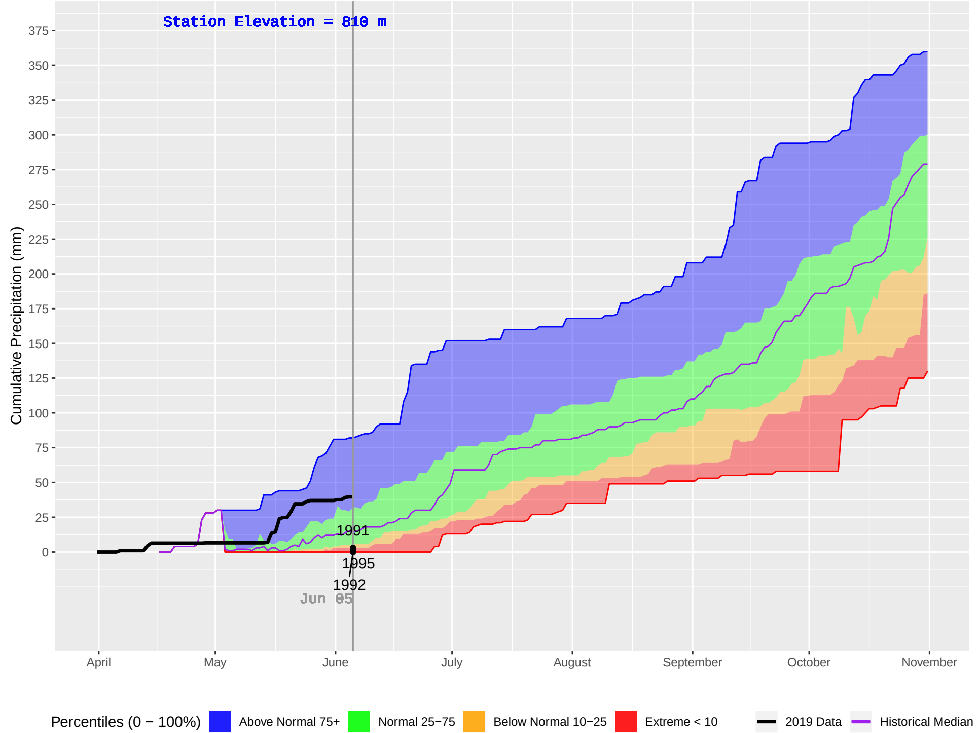
MCBRIDE LAKE (180) : Historical (1990–2018), Current (2019) Daily Cumulative Precipitation
